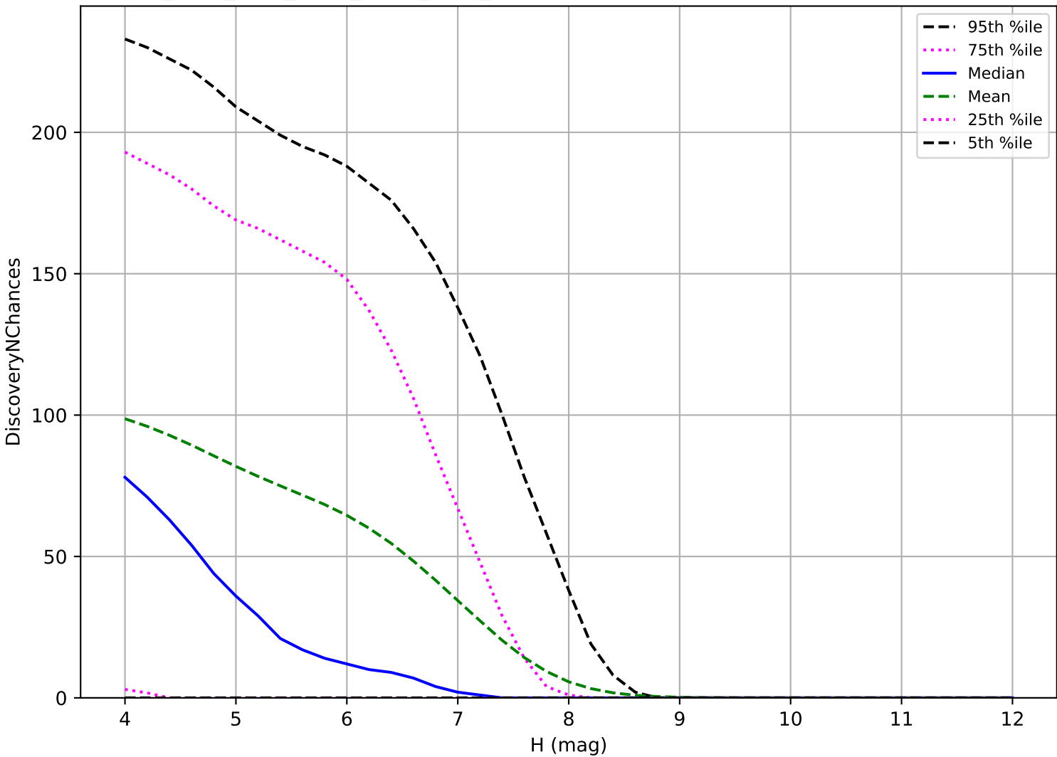
ddf_acor_sf25_lsf40_lsr50_v3.4_10yrs: TNO 3 pairs in 15 nights detection loss
