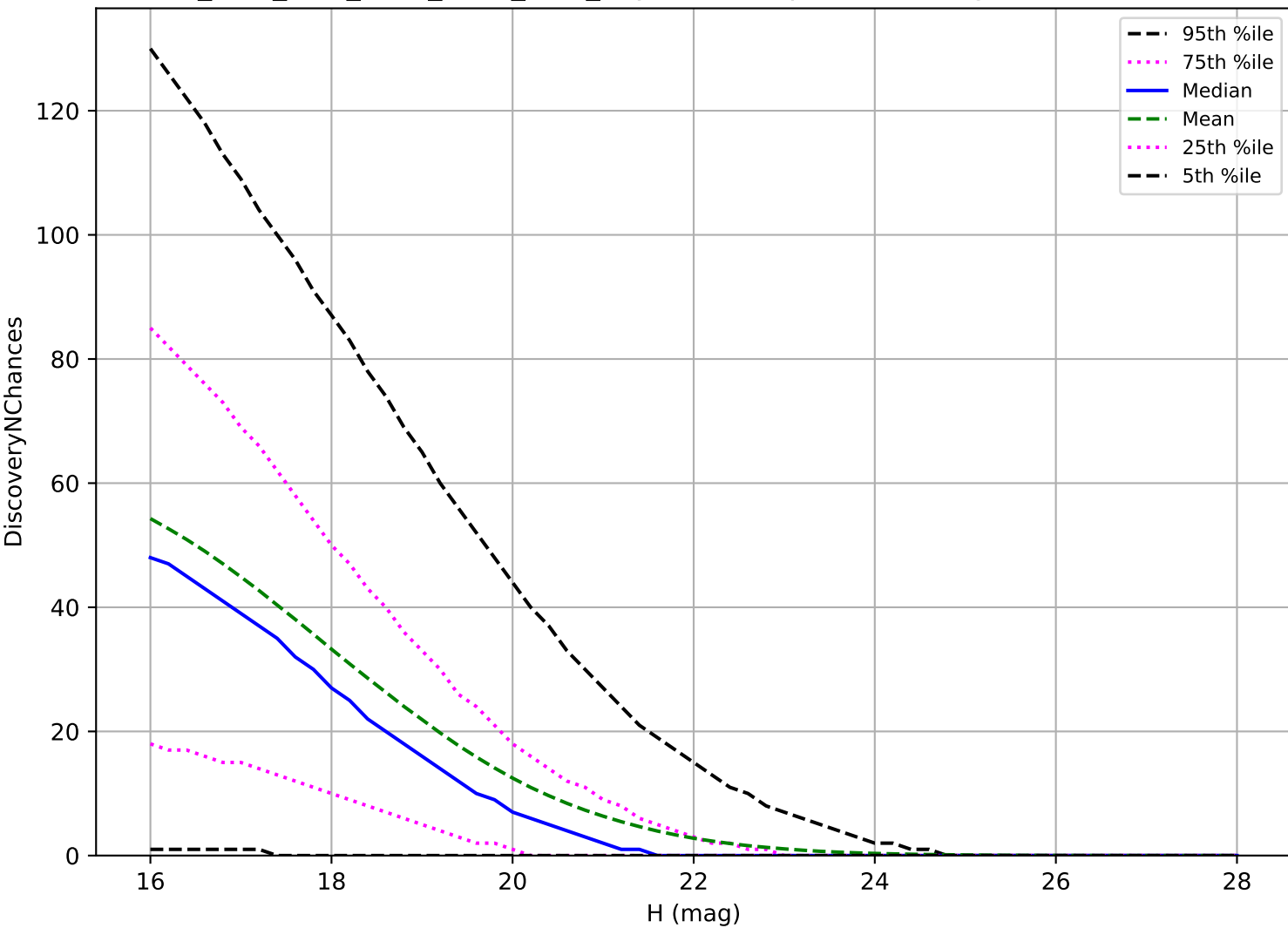
ddf_acor_sf25_lsf40_lsr50_v3.4_10yrs: PHA 3 pairs in 15 nights detection loss
