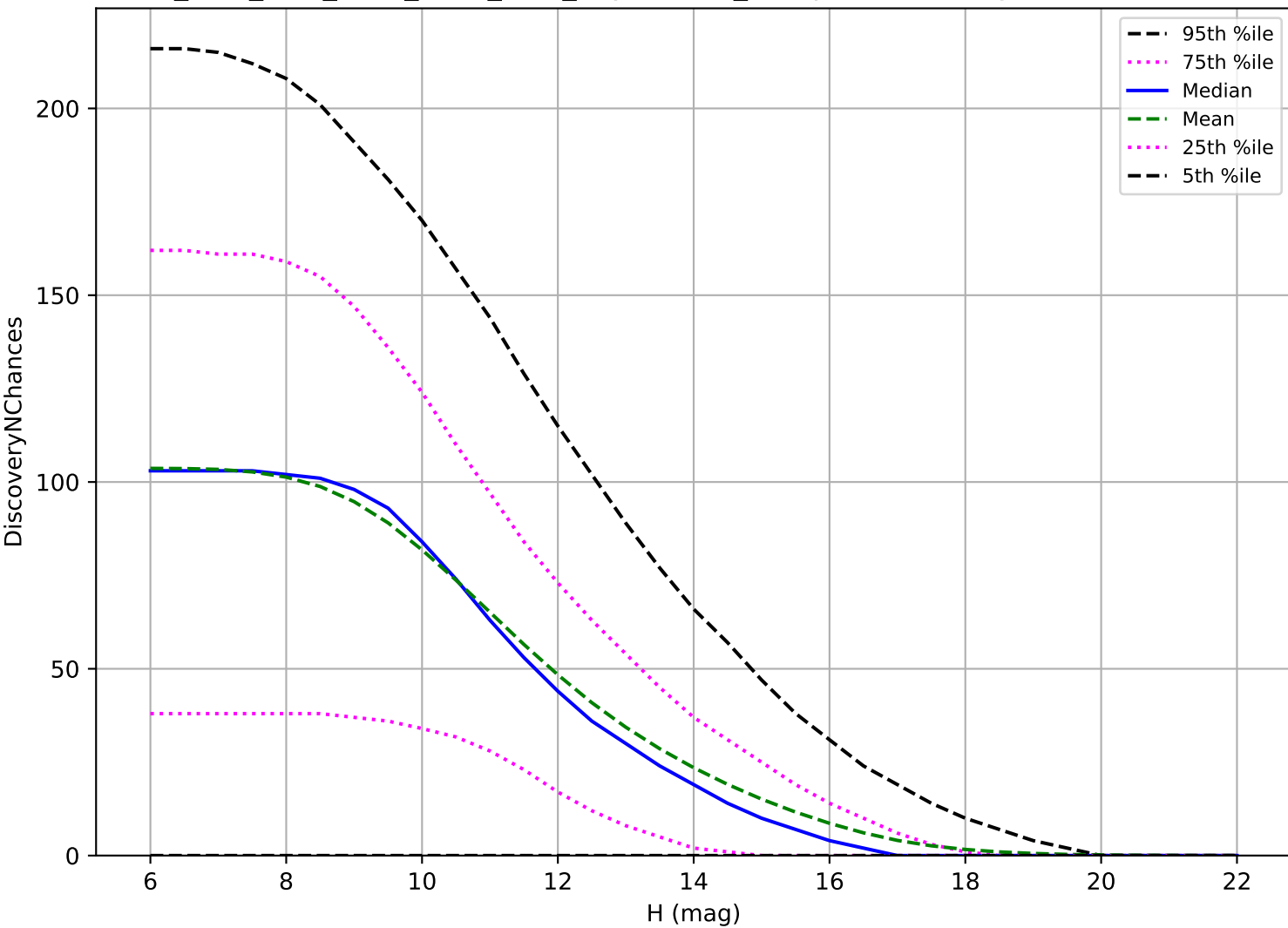
ddf_acor_sf25_lsf40_lsr50_v3.4_10yrs: OCC_r5 3 pairs in 15 nights detection loss
