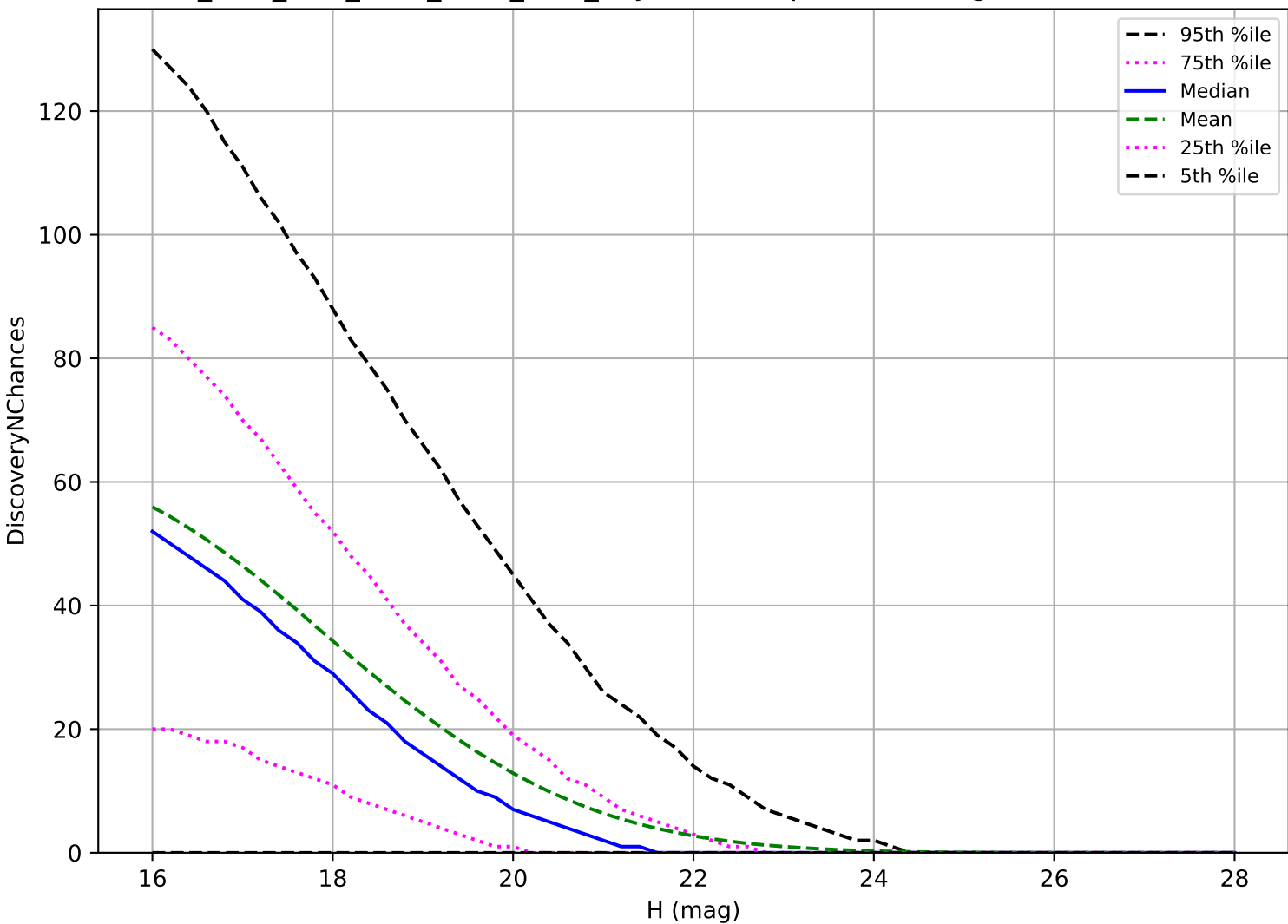
ddf_acor_sf25_lsf40_lsr50_v3.4_10yrs: NEO 3 pairs in 15 nights detection loss
