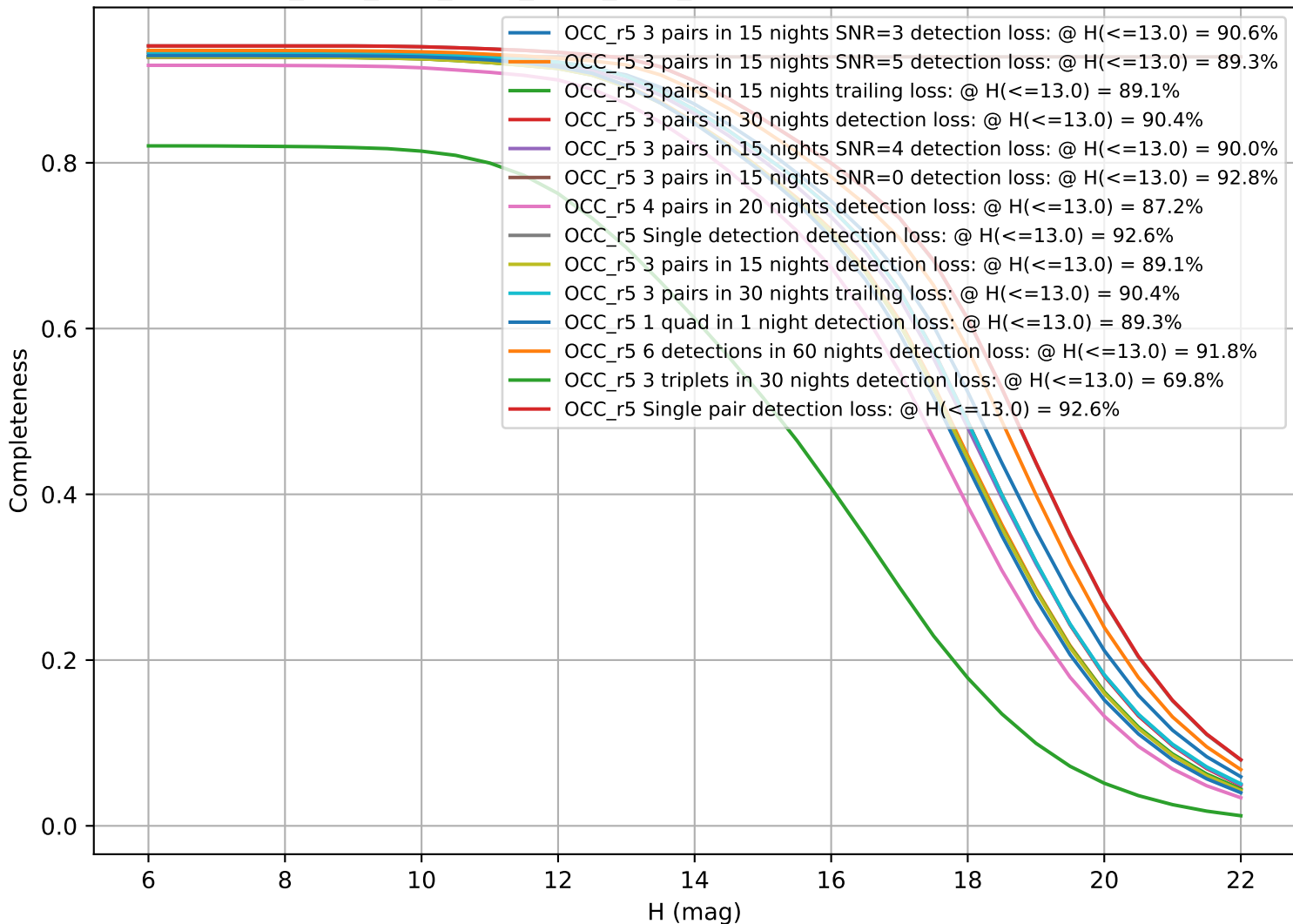
ddf_acor_sf25_lsf40_lsr50_v3.4_10yrs: CumulativeCompleteness
