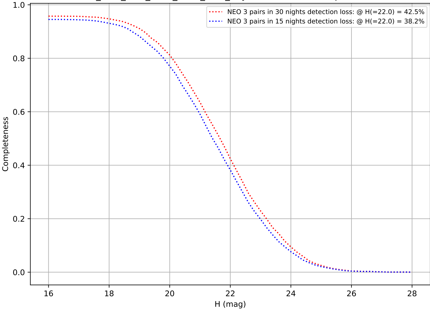
ddf_acor_sf25_lsf40_lsr50_v3.4_10yrs: DifferentialCompleteness
