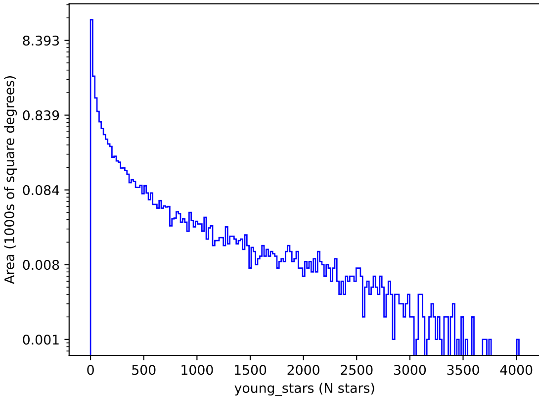
ddf_acor_sf25_lsf40_lsr50_v3.4_10yrs : young_stars
