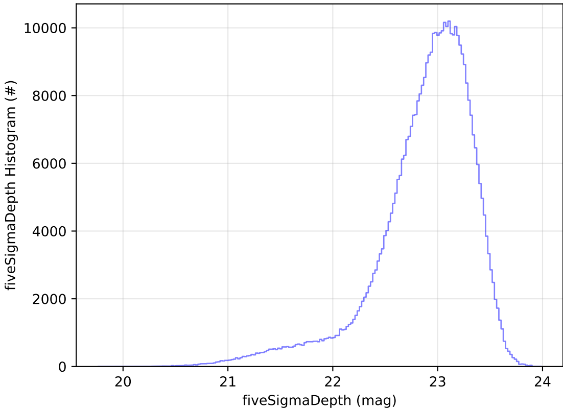
ddf_acor_sf25_lsf40_lsr50_v3.4_10yrs z: fiveSigmaDepth Histogram
