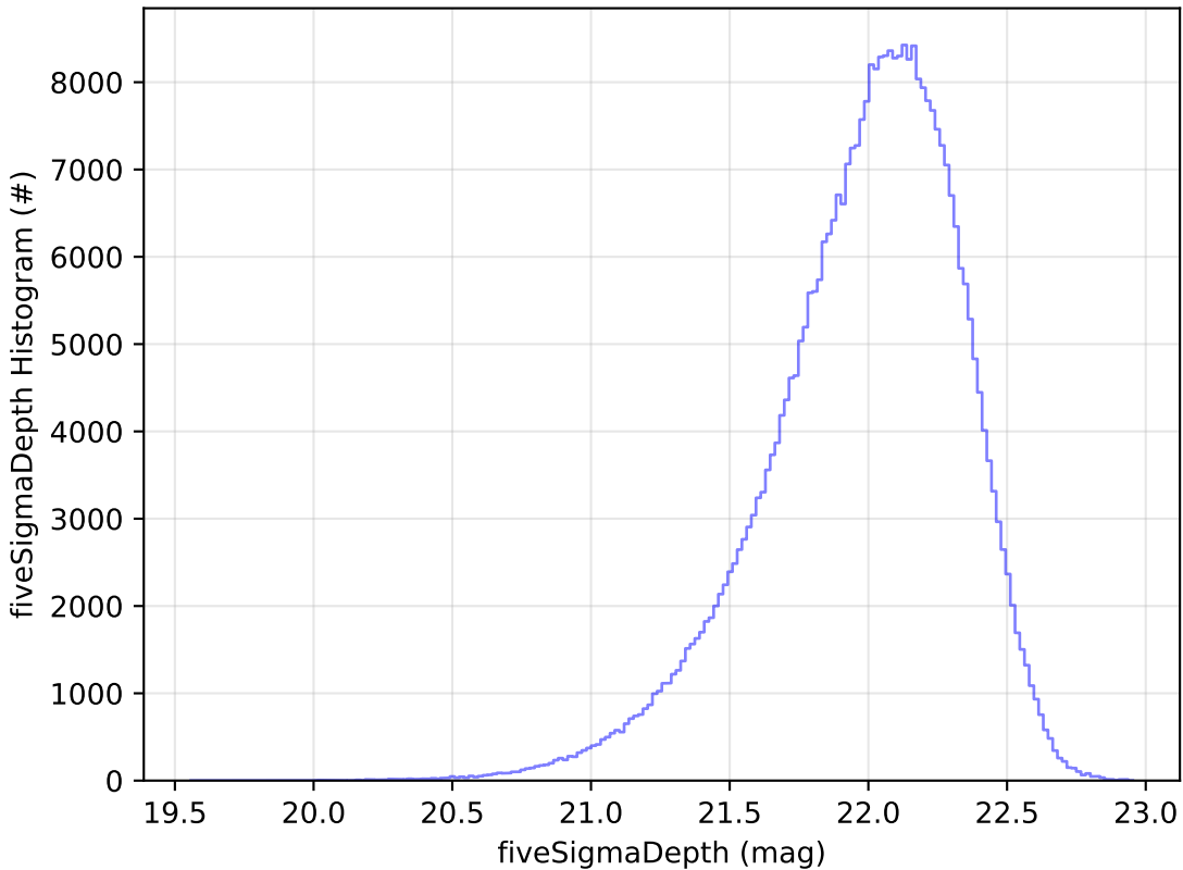
ddf_acor_sf25_lsf40_lsr50_v3.4_10yrs y: fiveSigmaDepth Histogram
