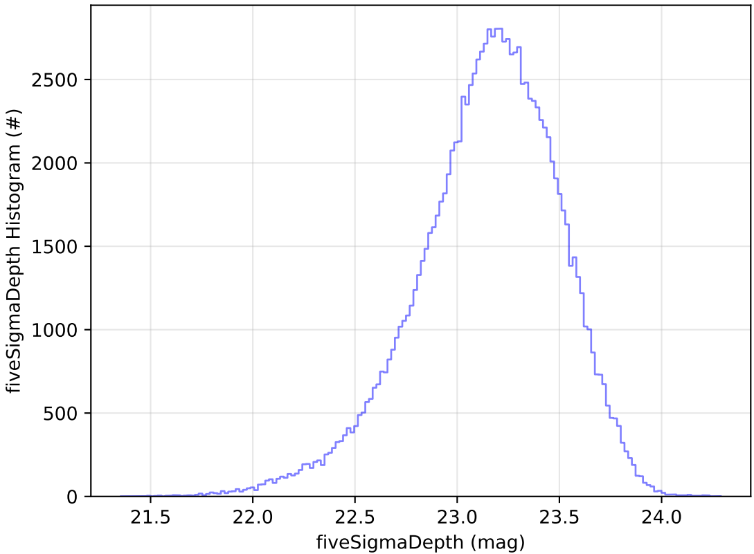
ddf_acor_sf25_lsf40_lsr50_v3.4_10yrs u: fiveSigmaDepth Histogram
