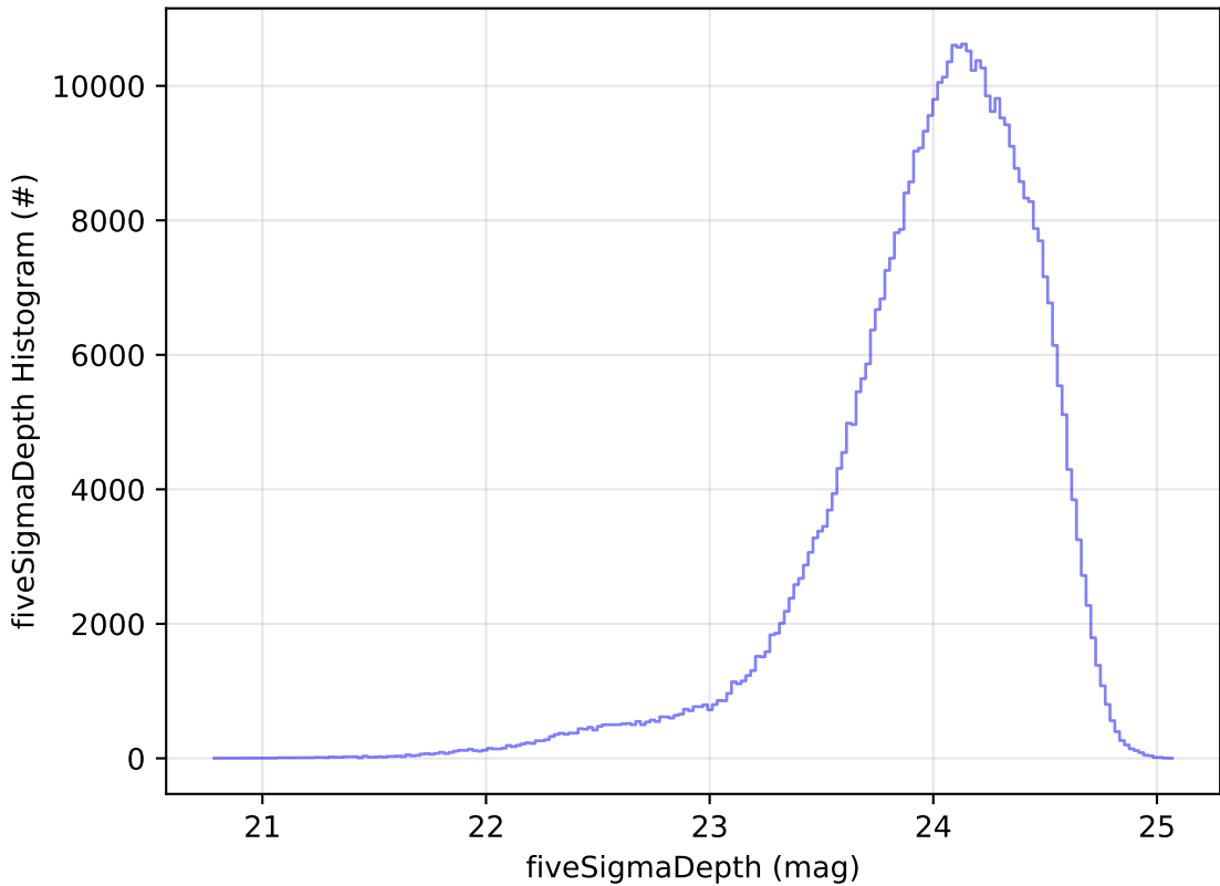
ddf_acor_sf25_lsf40_lsr50_v3.4_10yrs r: fiveSigmaDepth Histogram
