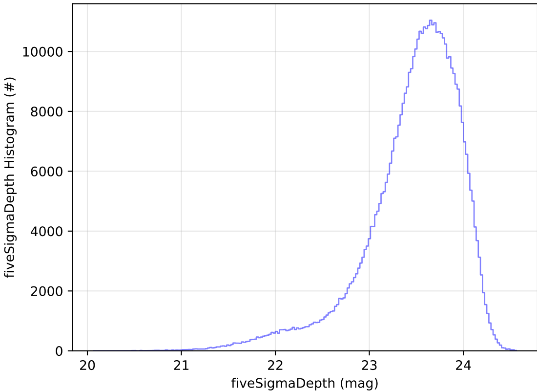
ddf_acor_sf25_lsf40_lsr50_v3.4_10yrs i: fiveSigmaDepth Histogram
