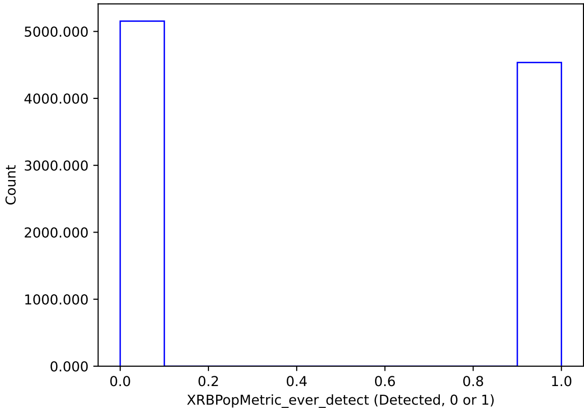
ddf_acor_sf25_lsf40_lsr50_v3.4_10yrs : XRBPoMetric_ever_detect
