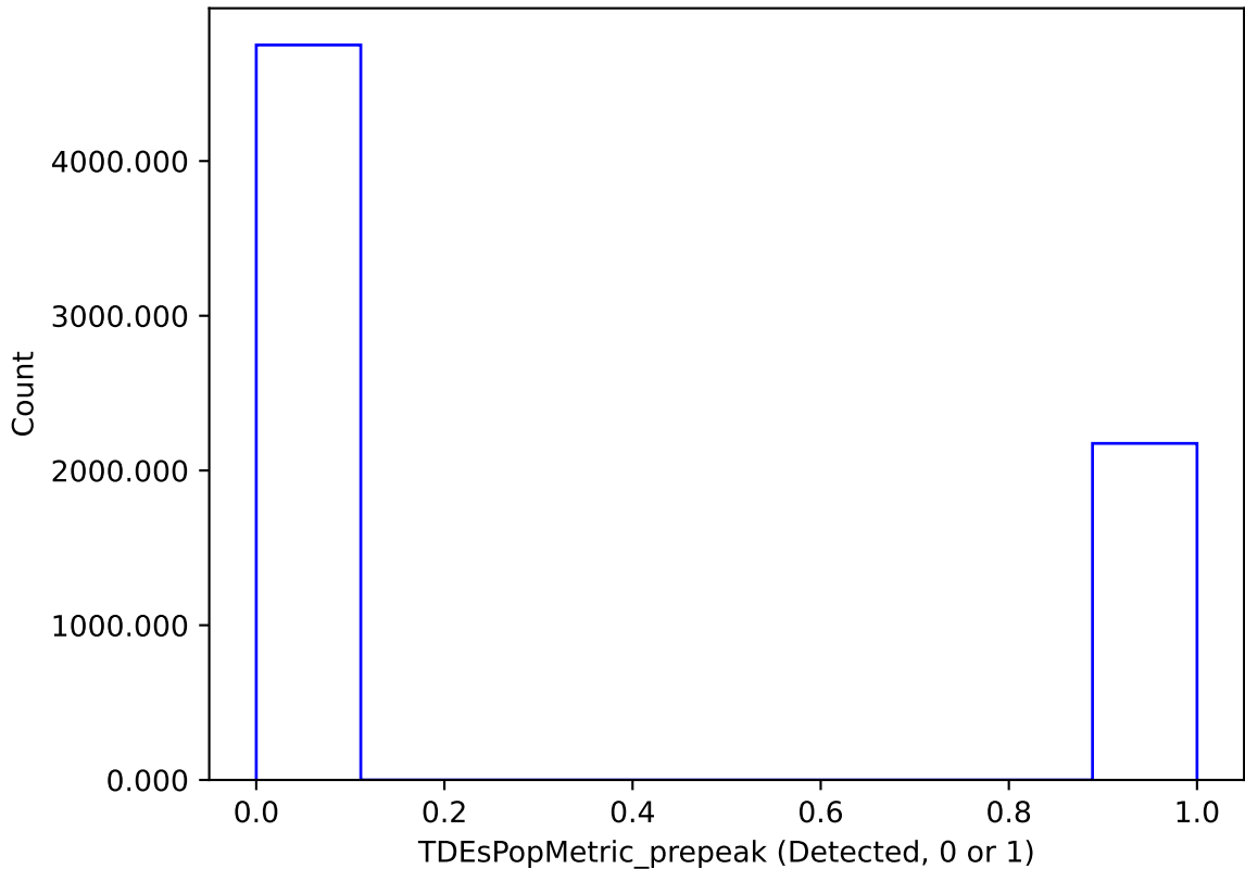
ddf_acor_sf25_lsf40_lsr50_v3.4_10yrs : TDEsPopMetric_prepeak
