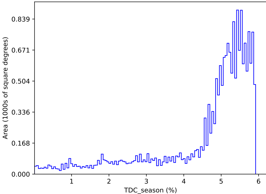
ddf_acor_sf25_lsf40_lsr50_v3.4_10yrs : TDC_season
