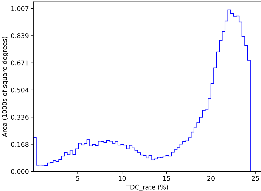
ddf_acor_sf25_lsf40_lsr50_v3.4_10yrs : TDC_rate
