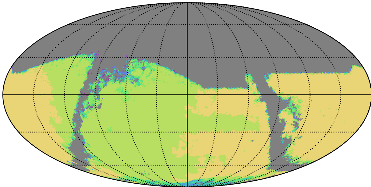
ddf_acor_sf25_lsf40_lsr50_v3.4_10yrs : TDC_campaign
