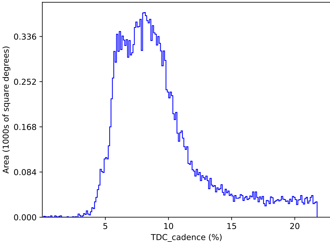
ddf_acor_sf25_ls40_lsr50_v3.4_10yrs : TDC_cadence
