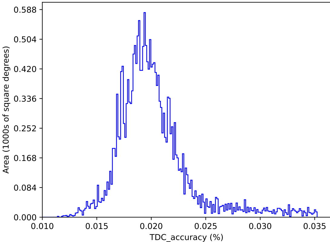
ddf_acor_sf25_lsf40_lsr50_v3.4_10yrs : TDC_accuracy
