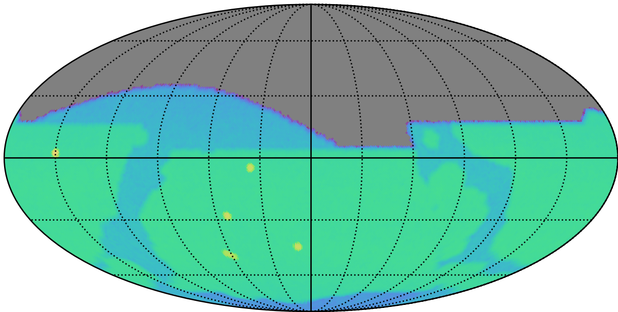
ddf_acor_sf25_lsf40_lsr50_v3.4_10yrs i: SurfaceBrightLimit
