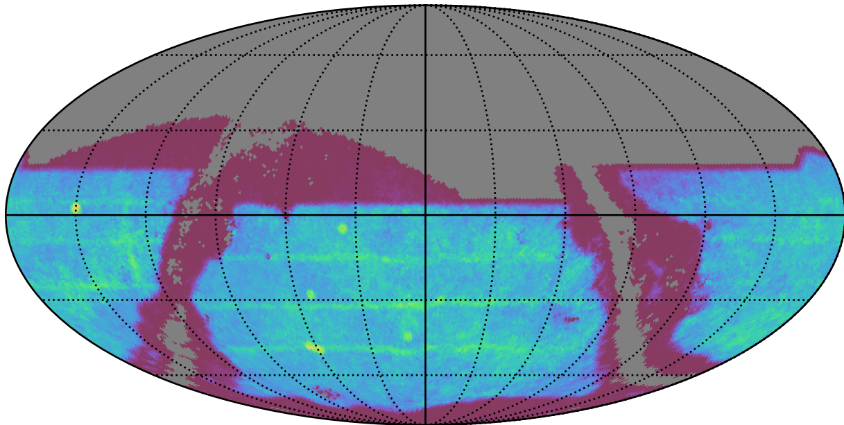
ddf_acor_sf25_lsf40_lsr50_v3.4_10yrs : SNSLMetric
