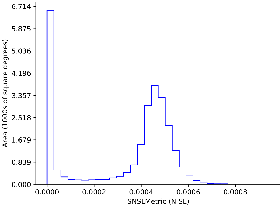
ddf_acor_sf25_lsf40_lsr50_v3.4_10yrs : SNSLMetric
