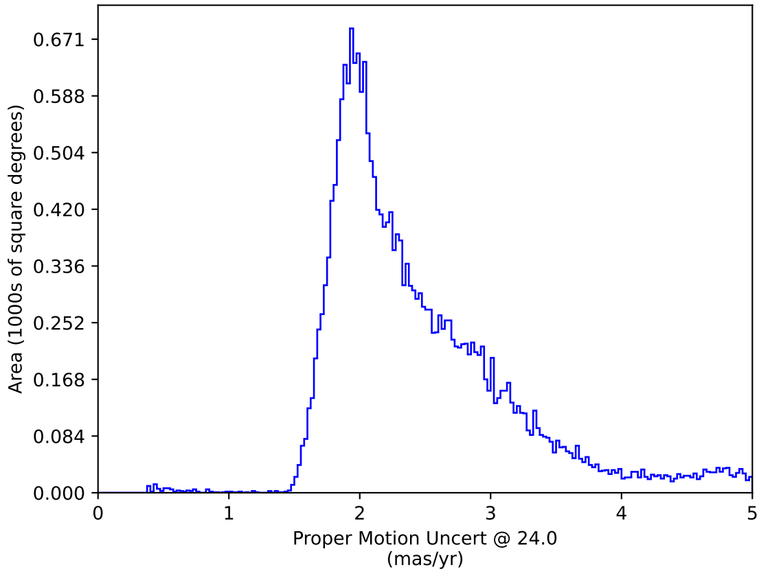
ddf_acor_sf25_lsf40_lsr50_v3.4_10yrs : Proper Motion Uncert @ 24.0
