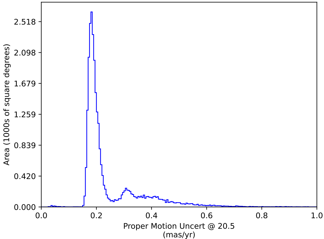
ddf_acor_sf25_lsf40_lsr50_v3.4_10yrs : Proper Motion Uncert @ 20.5
