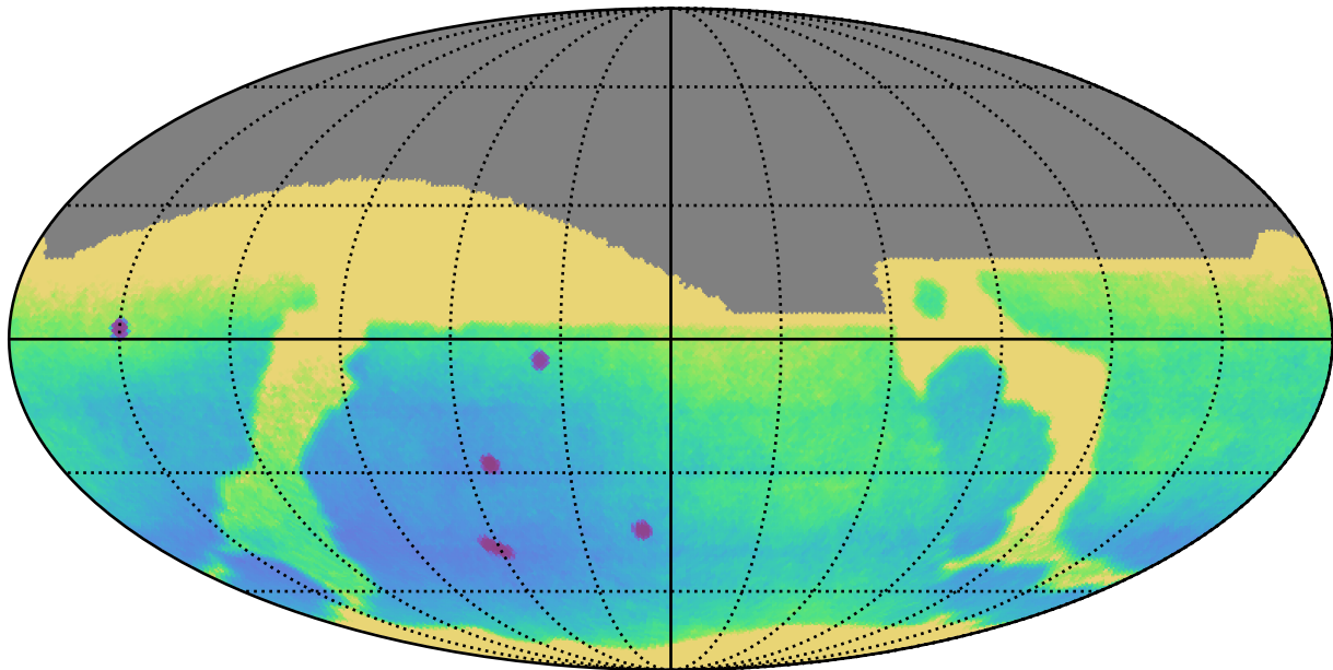
ddf_acor_sf25_lsf40_lsr50_v3.4_10yrs : Parallax Uncert @ 24.0
