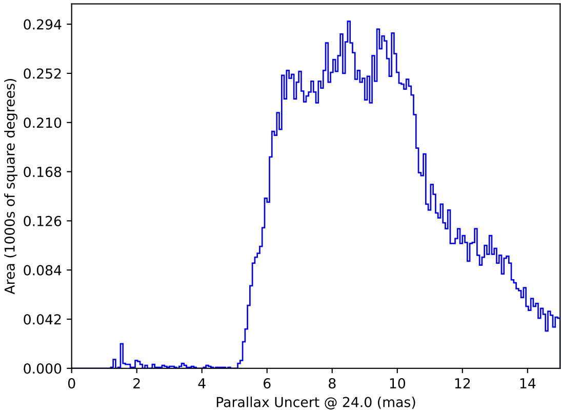
ddf_acor_sf25_lsf40_lsr50_v3.4_10yrs : Parallax Uncert @ 24.0
