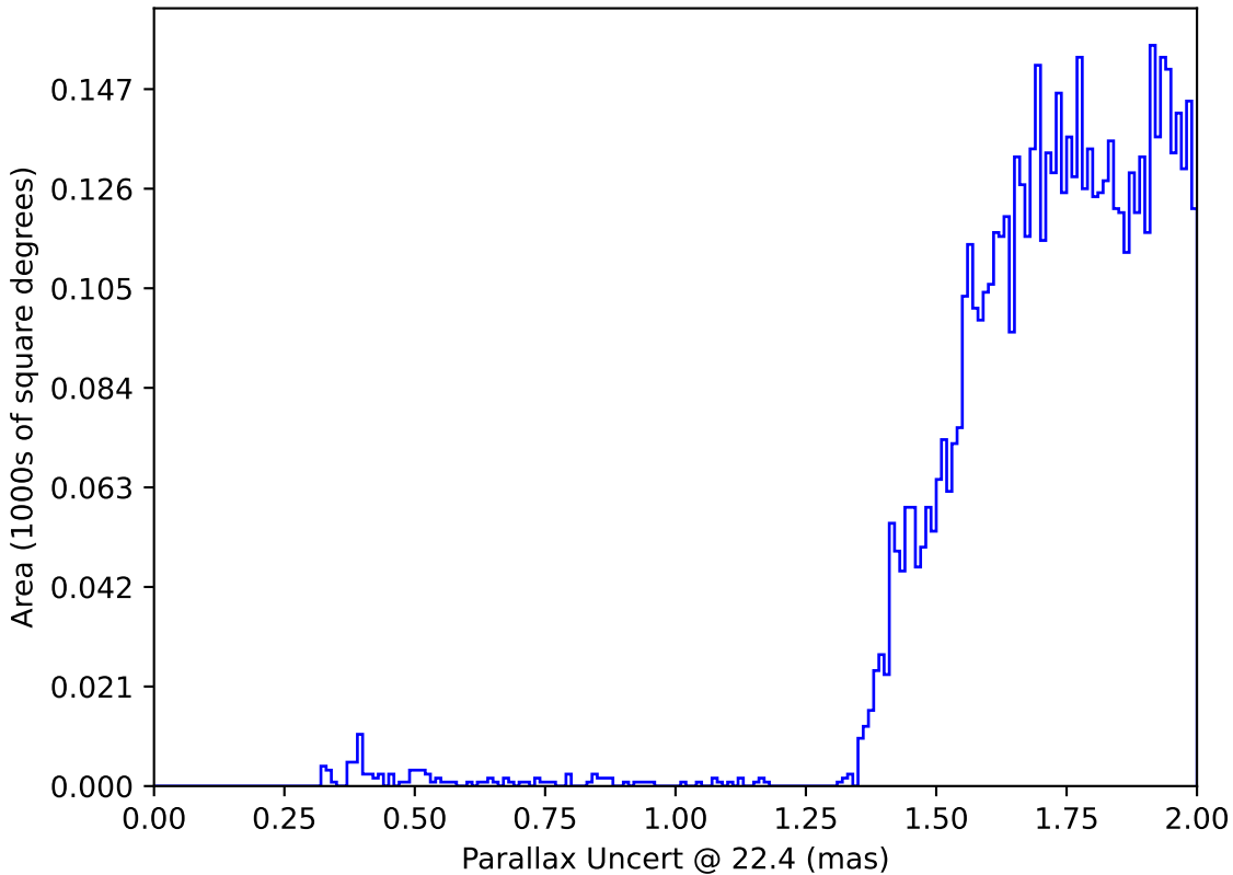
ddf_acor_sf25_lsf40_lsr50_v3.4_10yrs : Parallax Uncert @ 22.4
