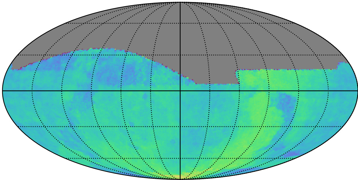
ddf_acor_sf25_lsf40_lsr50_v3.4_10yrs : Parallax Coverage @ 24.0
