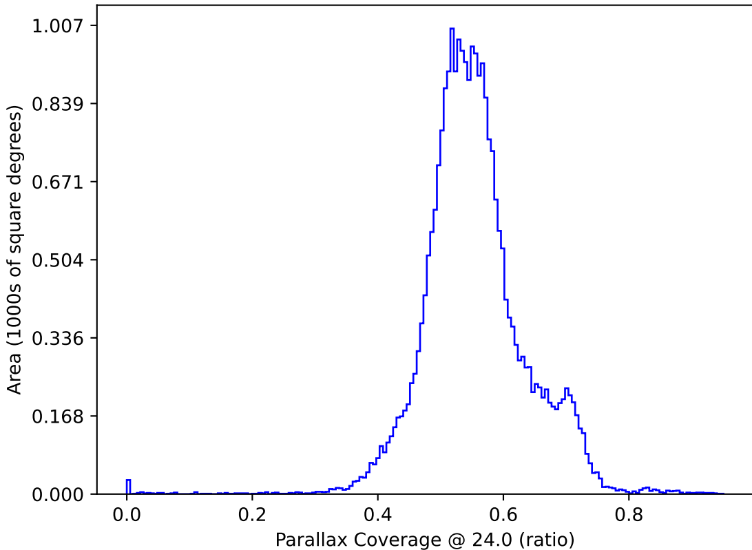
ddf_acor_sf25_lsf40_lsr50_v3.4_10yrs : Parallax Coverage @ 24.0
