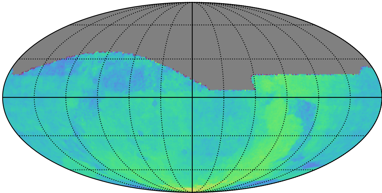
ddf_acor_sf25_lsf40_lsr50_v3.4_10yrs : Parallax Coverage @ 22.4
