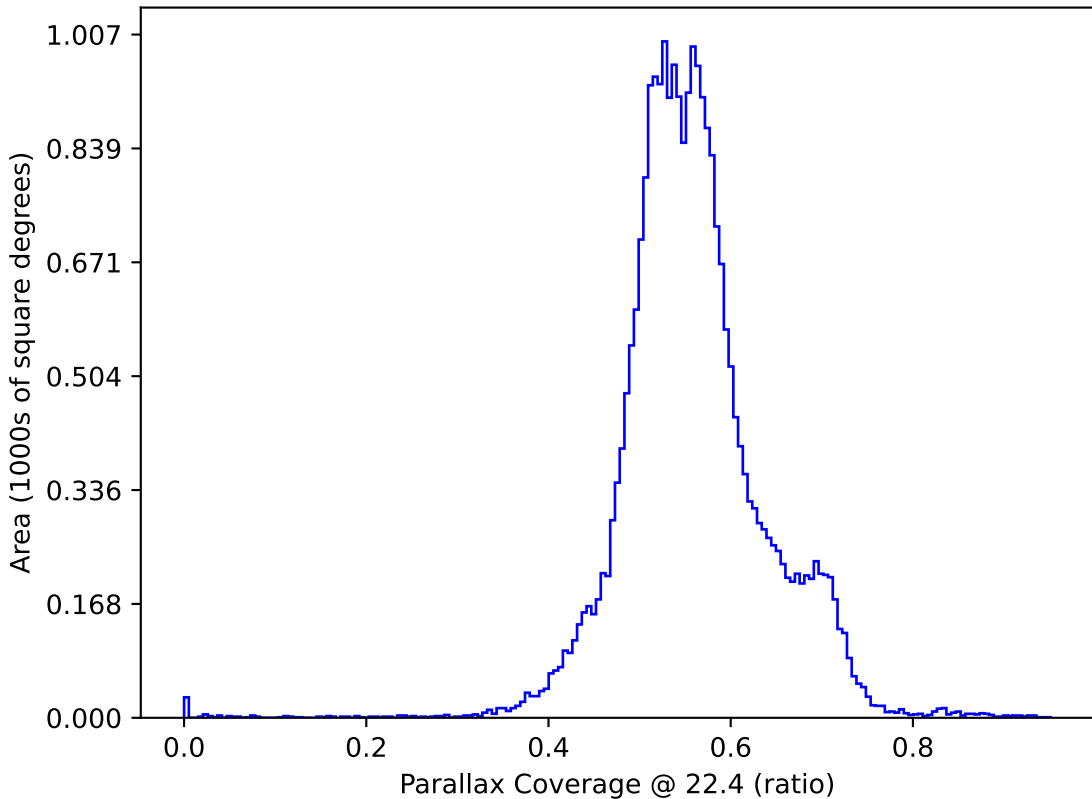
ddf_acor_sf25_lsf40_lsr50_v3.4_10yrs : Parallax Coverage @ 22.4
