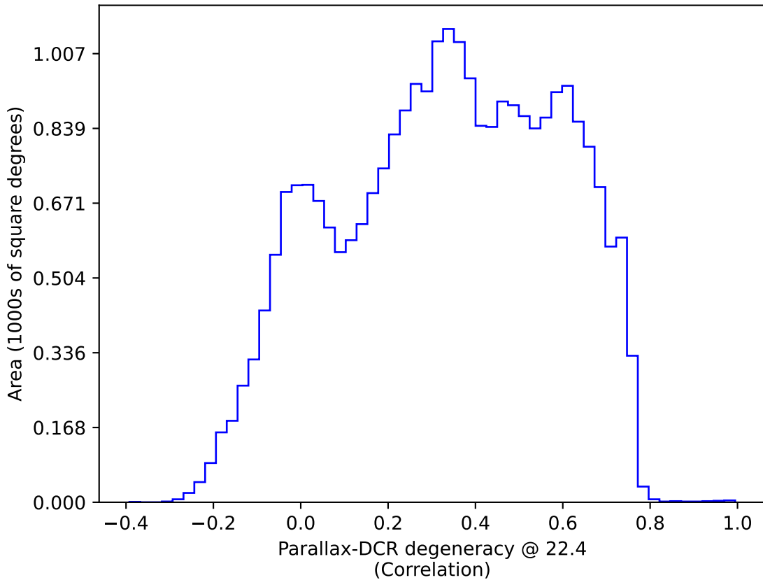
ddf_acor_sf25_lsf40_lsr50_v3.4_10yrs : Parallax-DCR degeneracy @ 22.4
