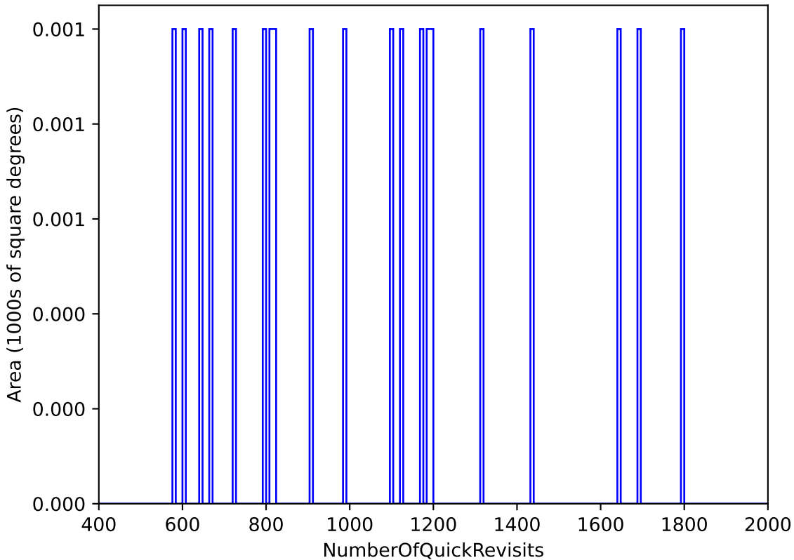
ddf_acor_sf25_lsf40_lsr50_v3.4_10yrs : NumberOfQuickRevisits
