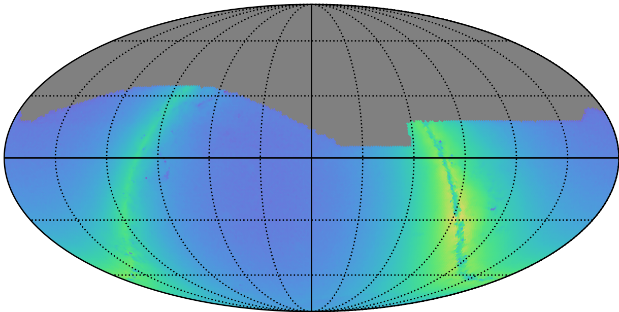
ddf_acor_sf25_lsf40_lsr50_v3.4_10yrs r: Nstars_no_crowding
