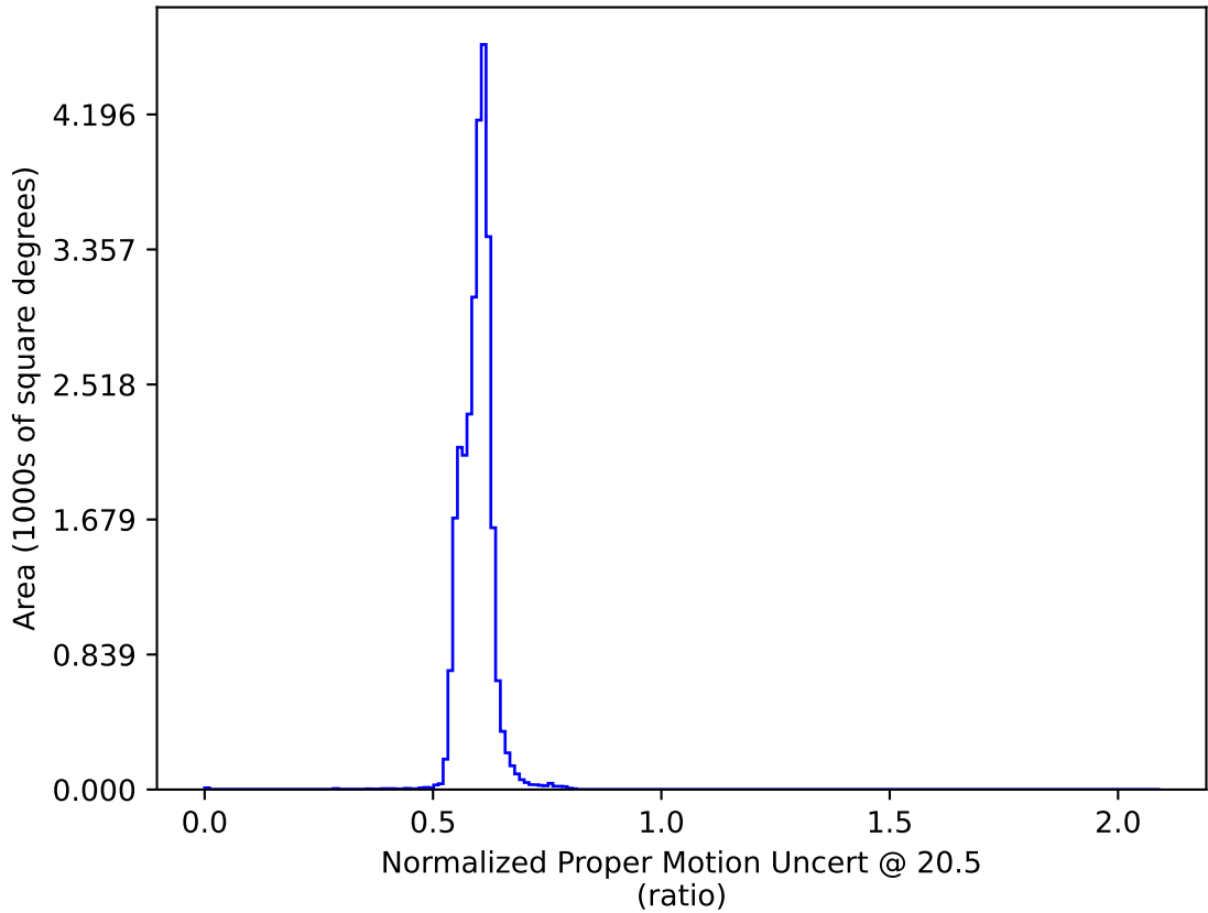
ddf_acor_sf25_lsf40_lsr50_v3.4_10yrs : Normalized Proper Motion Uncert @ 20.5
