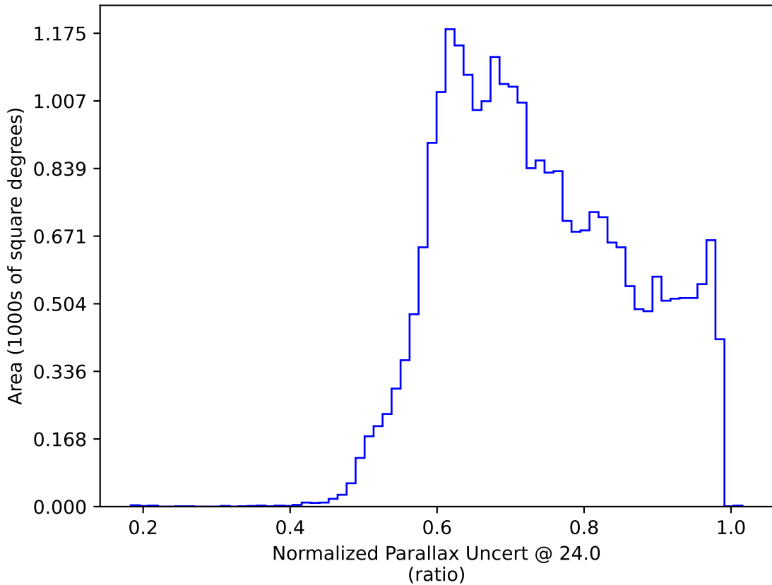
ddf_acor_sf25_lsf40_lsr50_v3.4_10yrs : Normalized Parallax Uncert @ 24.0
