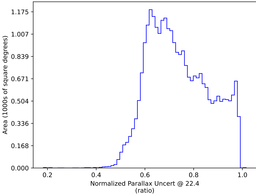
ddf_acor_sf25_lsf40_lsr50_v3.4_10yrs : Normalized Parallax Uncert @ 22.4
