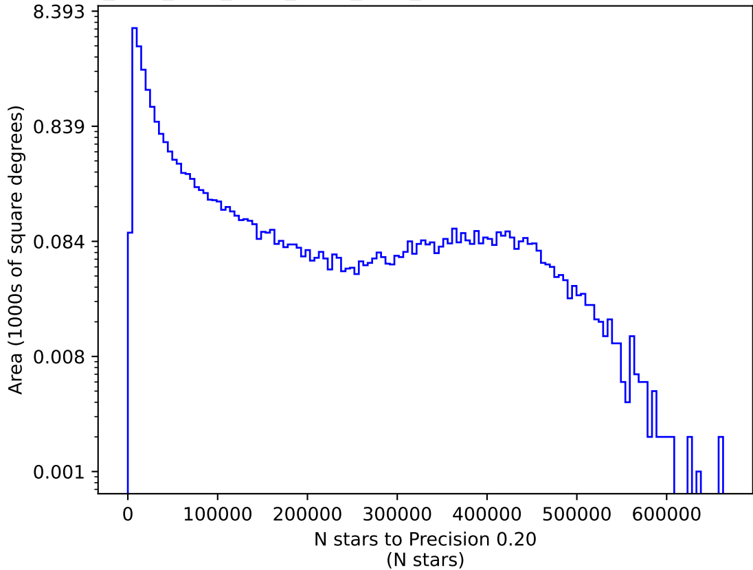
ddf_acor_sf25_lsf40_lsr50_v3.4_10yrs z: N stars to Precision 0.20
