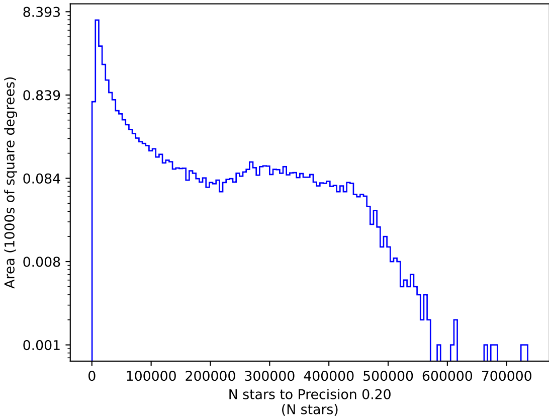
ddf_acor_sf25_lsf40_lsr50_v3.4_10yrs y: N stars to Precision 0.20
