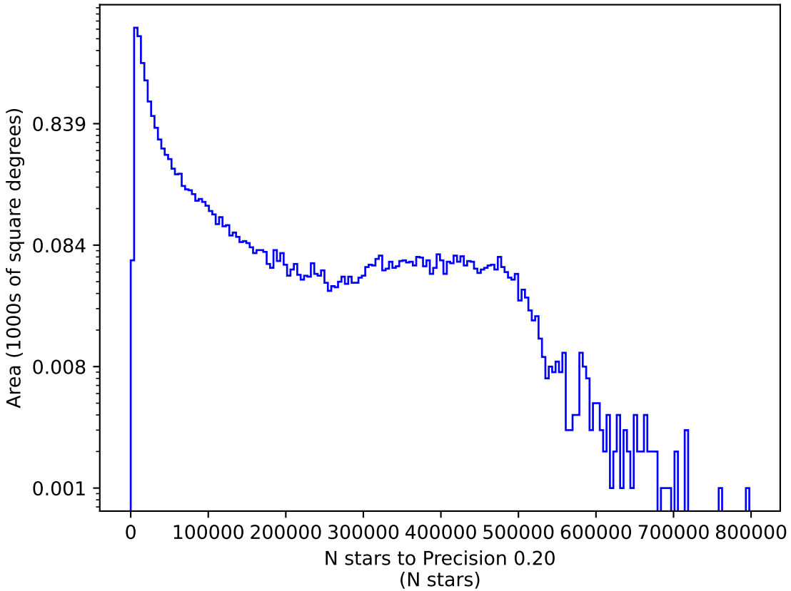
ddf_acor_sf25_lsf40_lsr50_v3.4_10yrs r: N stars to Precision 0.20
