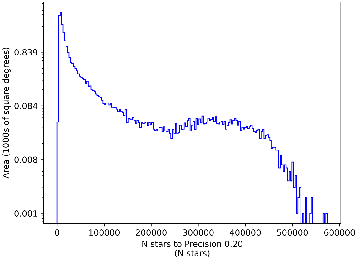
ddf_acor_sf25_lsf40_lsr50_v3.4_10yrs g: N stars to Precision 0.20
