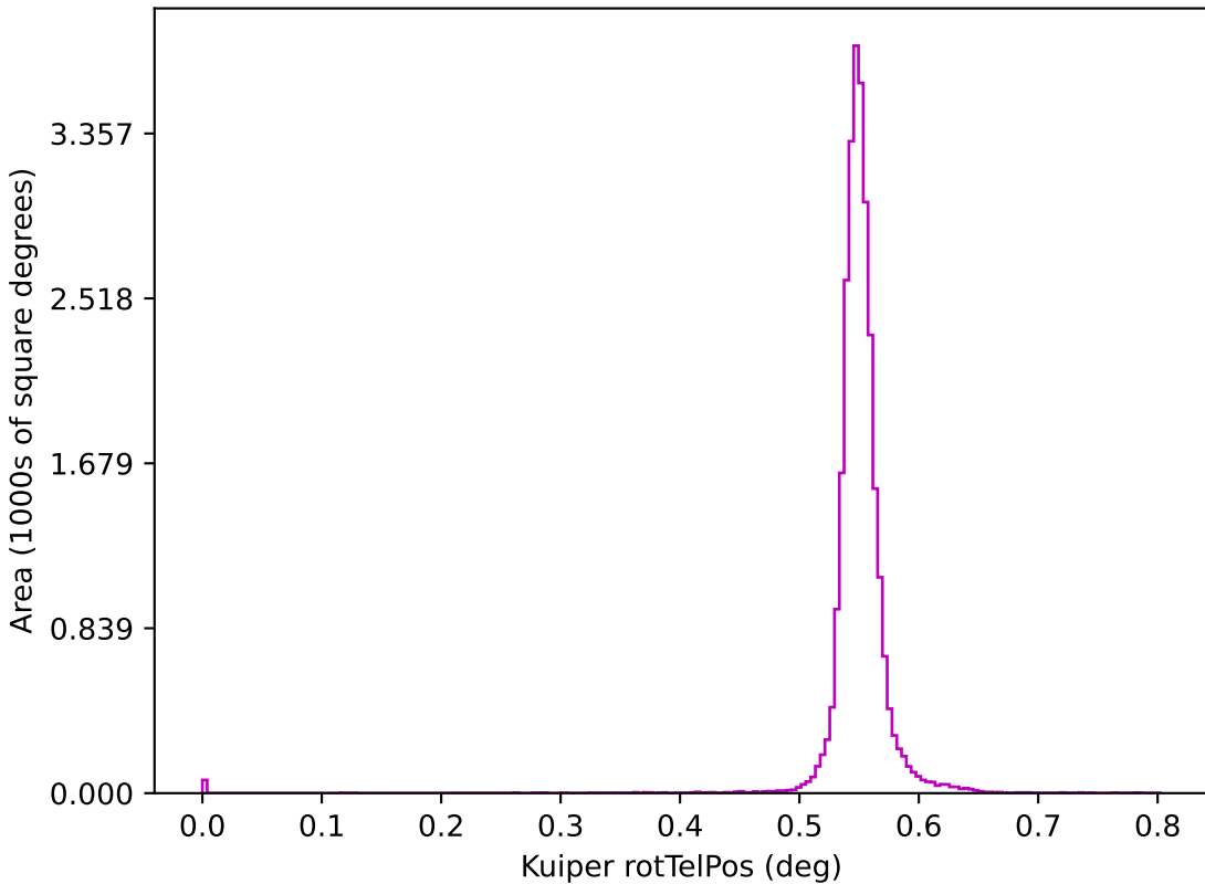
ddf_acor_sf25_lsf40_lsr50_v3.4_10yrs z: Kuiper rotTelPos
