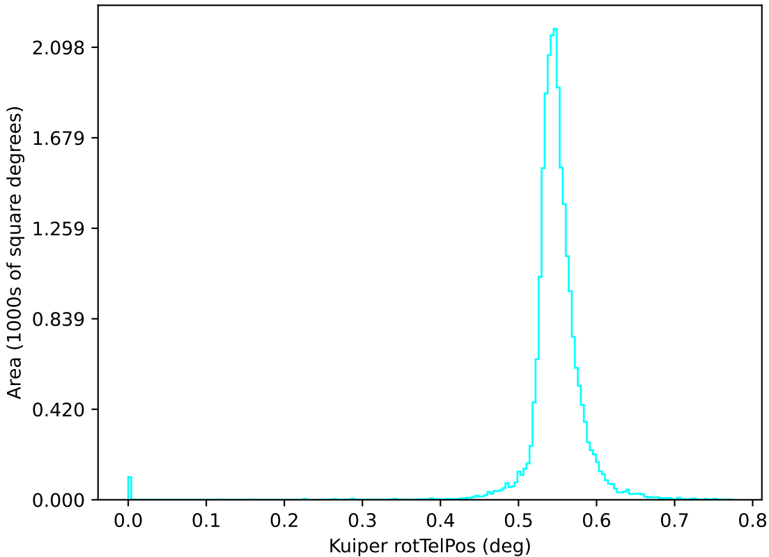
ddf_acor_sf25_lsf40_lsr50_v3.4_10yrs u: Kuiper rotTelPos
