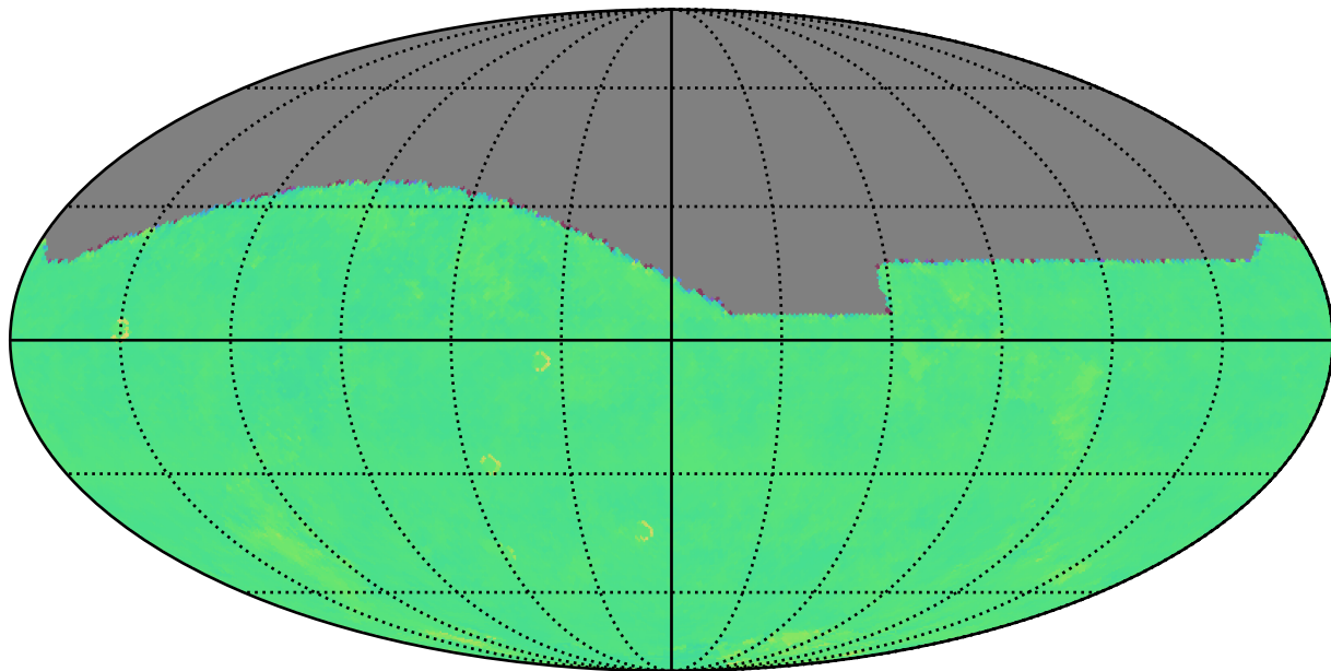
ddf_acor_sf25_lsf40_lsr50_v3.4_10yrs r: Kuiper rotTelPos
