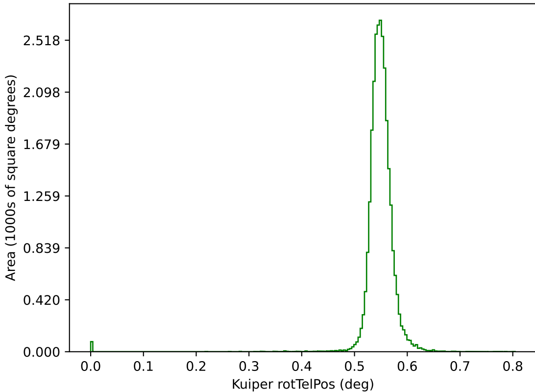
ddf_acor_sf25_ls40_lsr50_v3.4_10yrs g: Kuiper rotTelPos
