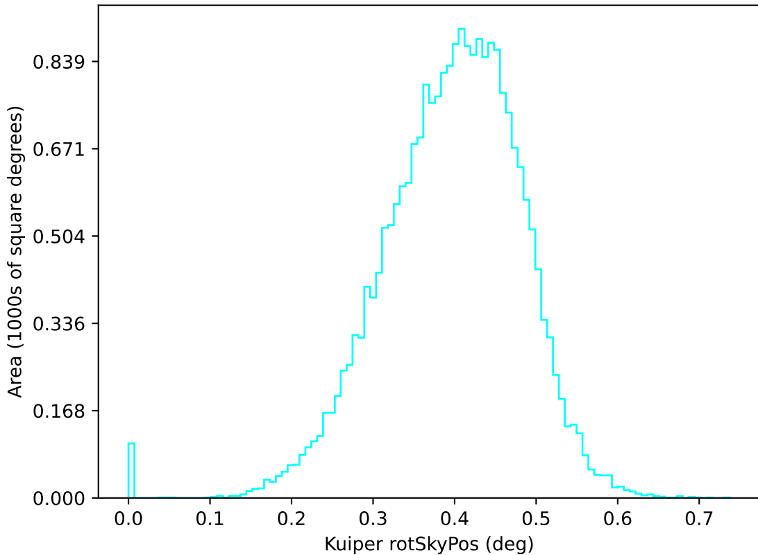
ddf_acor_sf25_lsf40_lsr50_v3.4_10yrs u: Kuiper rotSkyPos
