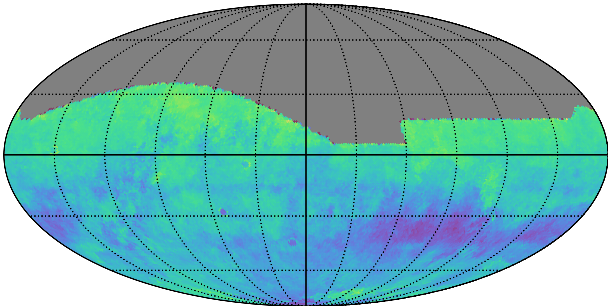
ddf_acor_sf25_lsf40_lsr50_v3.4_10yrs r: Kuiper rotSkyPos
