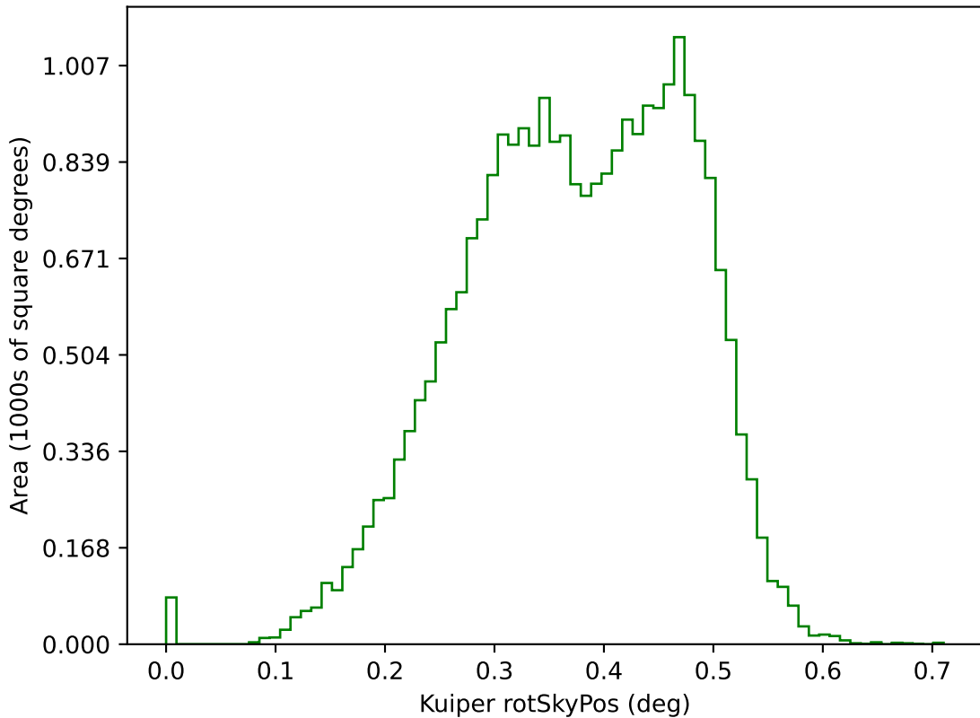
ddf_acor_sf25_lsf40_lsr50_v3.4_10yrs g: Kuiper rotSkyPos
