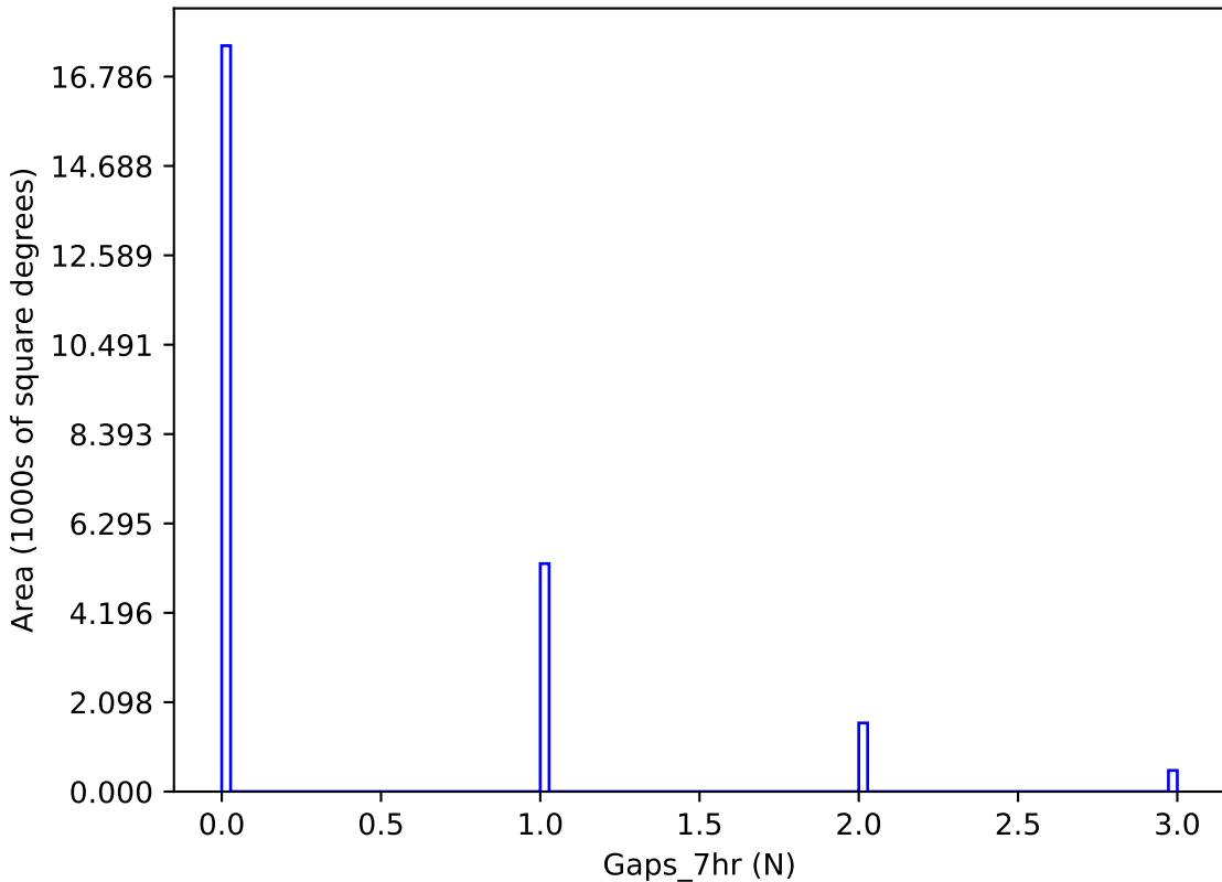
ddf_acor_sf25_ls40_lsr50_v3.4_10yrs y band: Gaps_7hr
