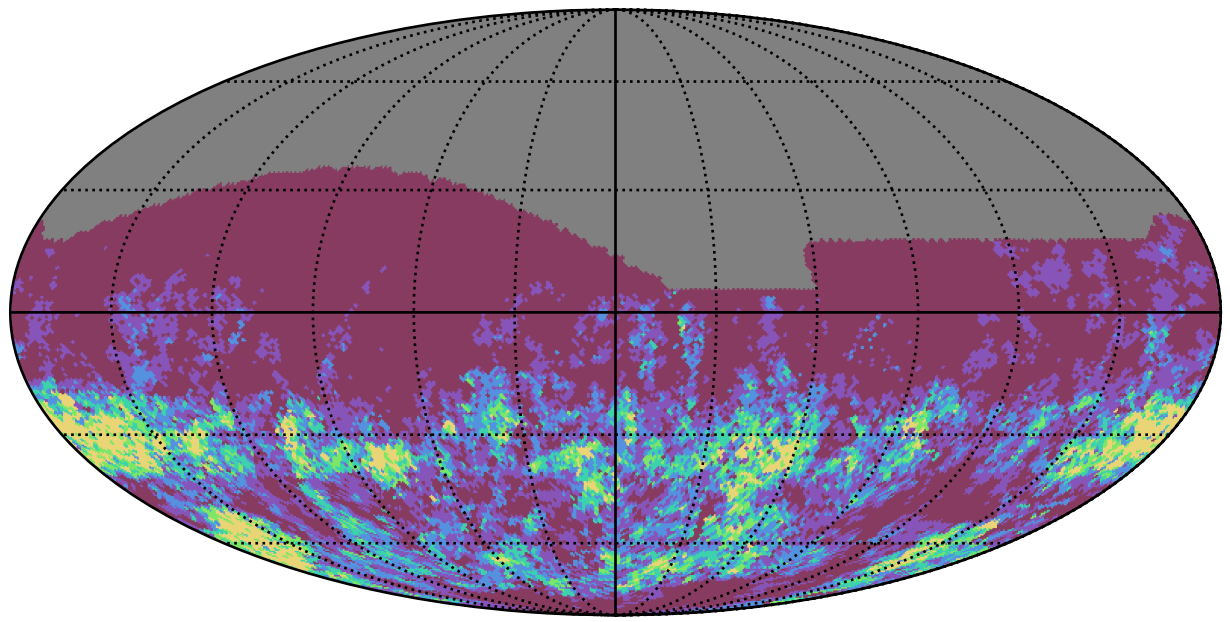
ddf_acor_sf25_lsf40_lsr50_v3.4_10yrs r band: Gaps_7hr
